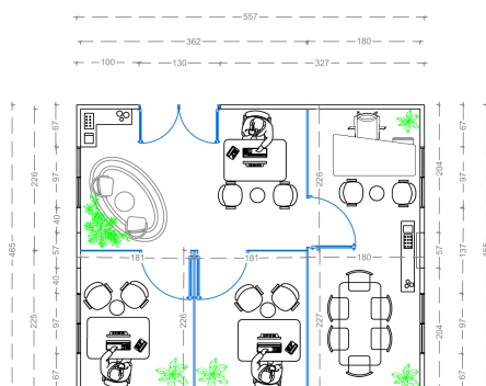
Foldable Caravan 2 — Workstations · Meeting Room · Lounge · Conference Room — Total 5,570mm × 4,650mm
