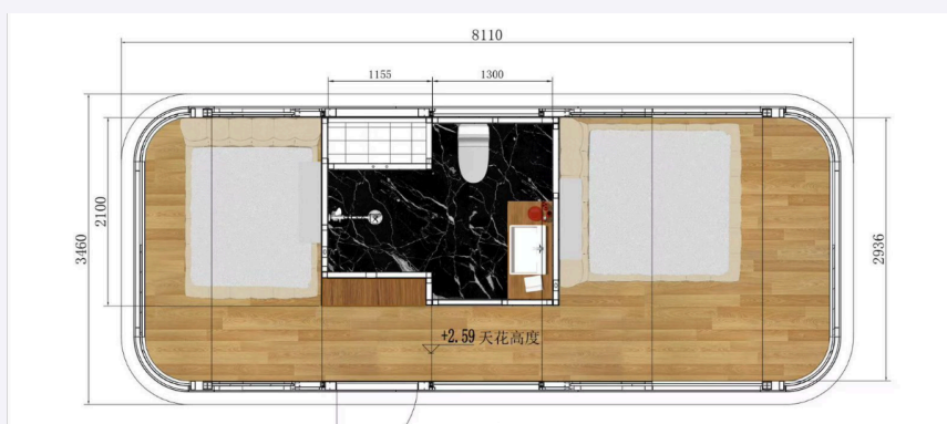
1st Generation 8.11m Modular Space Capsule — Twin Bedrooms · Central Bathroom — Total 8,110mm × 3,460mm
