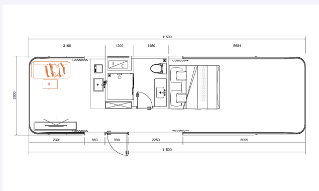
Space Capsule 11.5m — Lounge · Kitchenette · Bathroom · Bedroom — Total 11,500mm × 3,300mm
